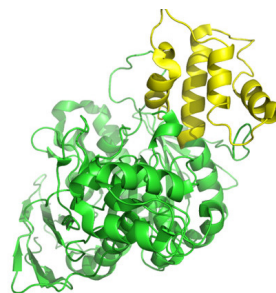
BSSL molekylen
